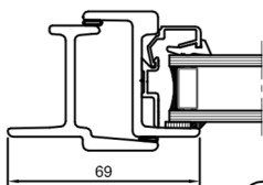
Unequal Leg Opening Outward
