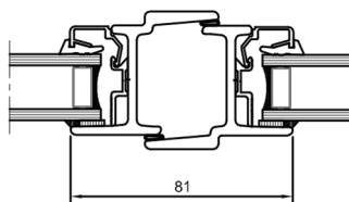
Typical Meeting Stile
