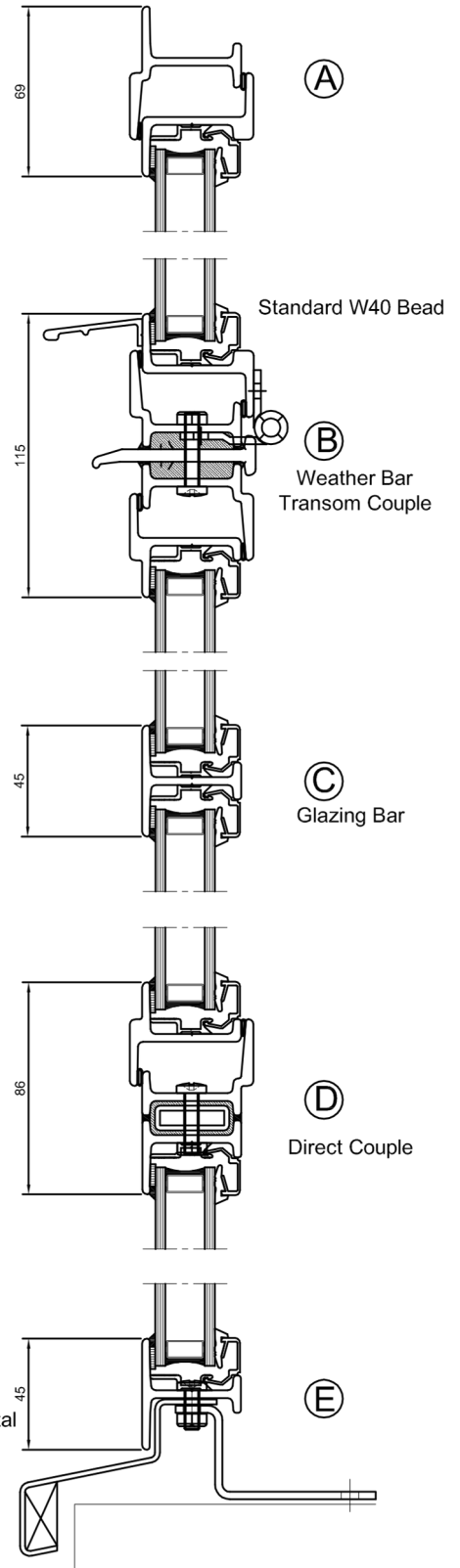
Alternate Glazing Bar
