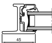
Fixed Light Section
